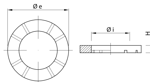
8 x 2.00 mm SLOT
